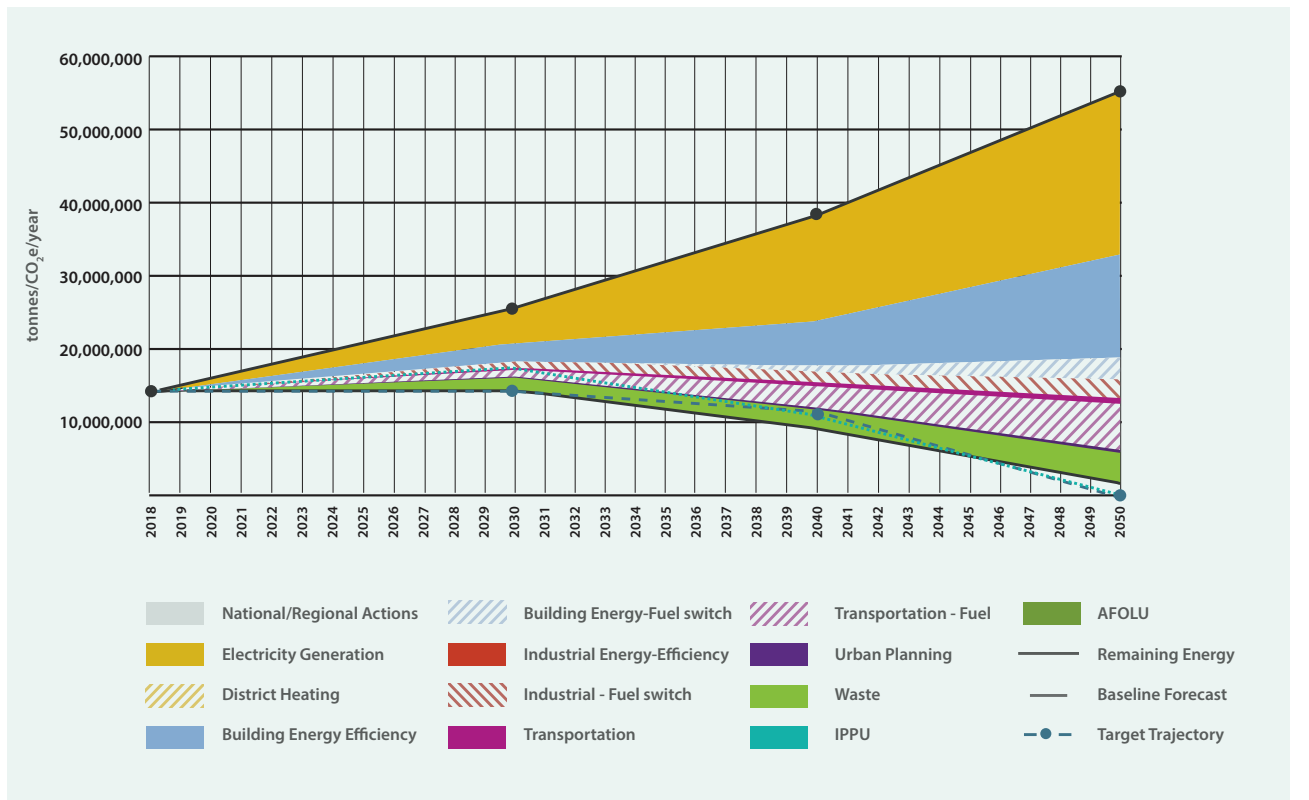
Figure 53: Pathways for Extended Scenario
