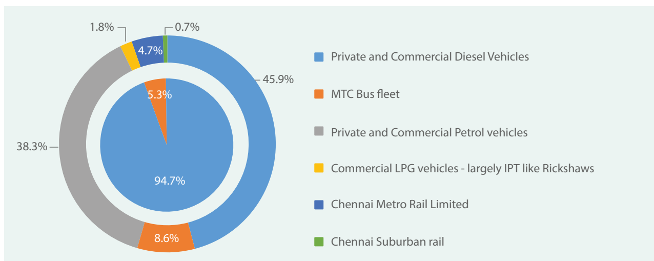
Figure 47: CO 2 Emissions from Transportation Sector
