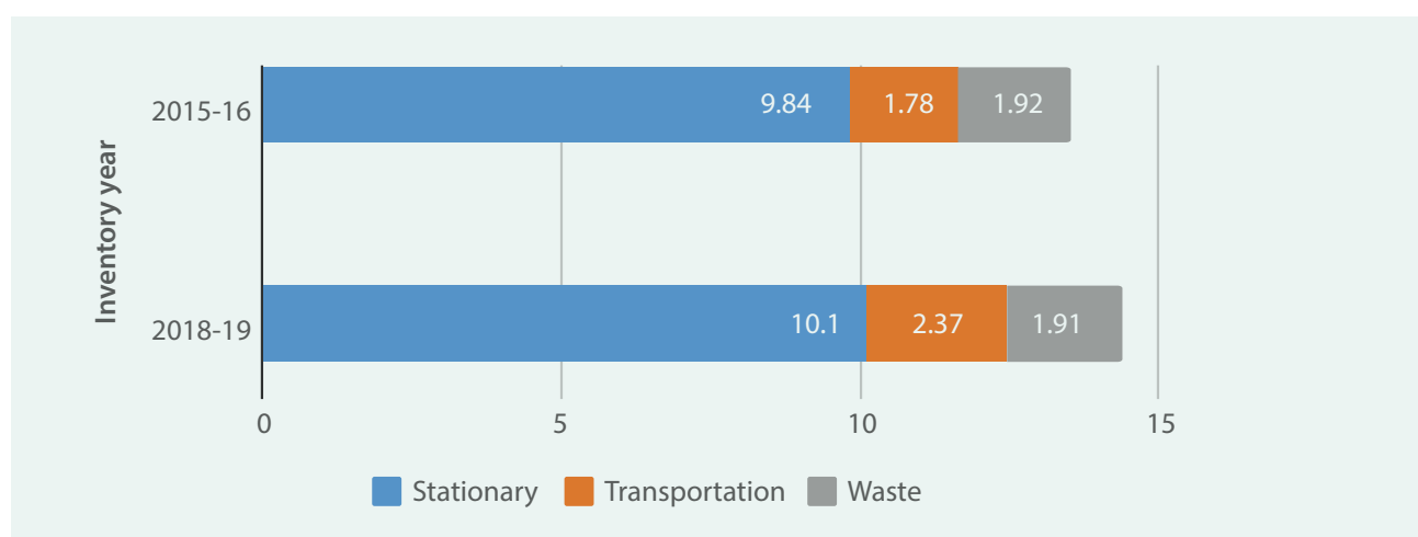
Figure 44: Change in Emissions from 2015-16 to 2018-19
